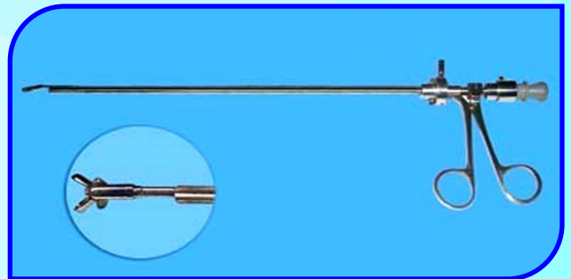
Biopsy Forcep
